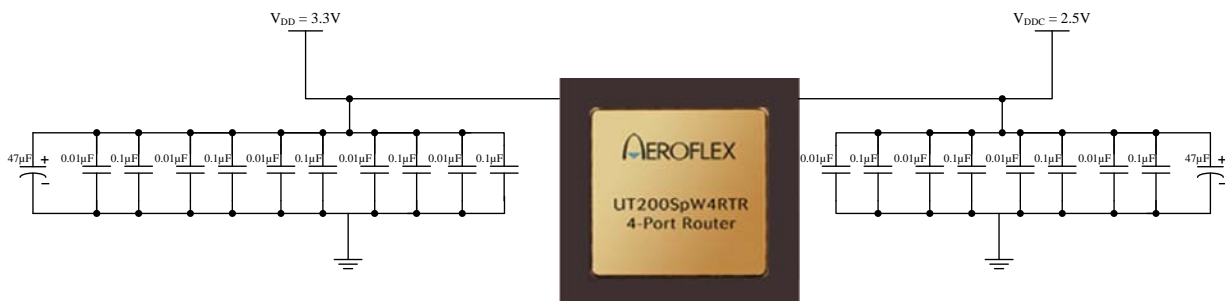
Figure 1. Example Decoupling Scheme
